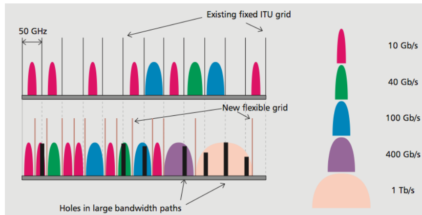
Figure 1.4: Flexible grid to support different bit rate demands [3].
