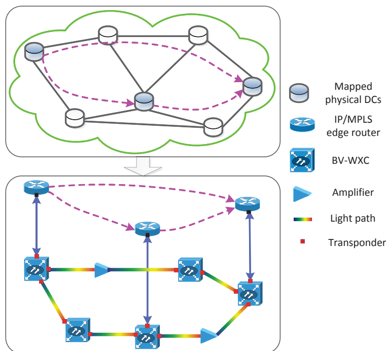
Figure 5.3 Multi-layer routing in the Cloud platform.
